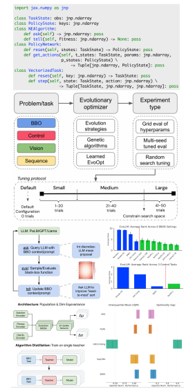
Figure 6: Our works on evolution strategy. Top-to-bottom: EvoJAX [16], NeuroEvoBench [10], EvoLLM [11] and EvoTransformer [12].
